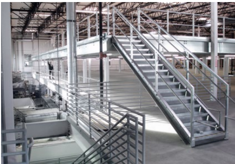
OSHA Mezzanine/Platform Guardrails
