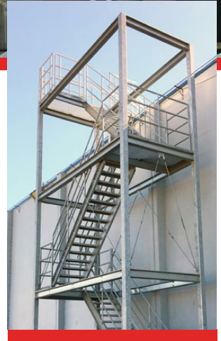
Stair Towers Guardrails
